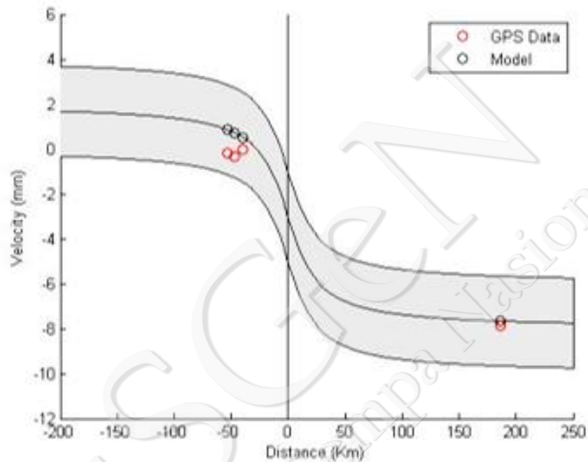
Gambar IV-23. Segmen Suliti-Siulak
