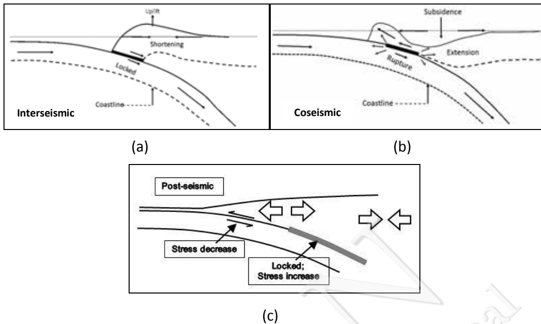
Gambar IV-1. Mekanisme fase gempa: (a) interseismic , (b) coseismic , (c) postseismic (digambar ulang berdasarkan Savage 1983)
