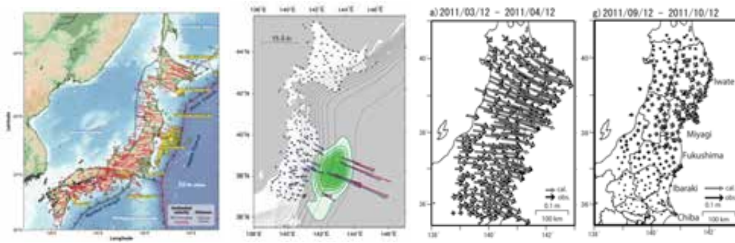
Figure 2.7. (Left) Horizontal velocity at onshore and offshore GPS in Japan w.r.t to Eurasia plate in Gambar IV-4. (kiri) Fase interseismik (sebelum) pada September 2007 – Februari 2011 (Nishimura dkk., 2014); (dua) Fase koseismik pada gempa Tohoku Jepang 2011 M9.0 (Hashimoto dkk., 2012); arah deformasi (Nishimura et al., 2011); (tengah) Fase postseismik (setelah gempa) (Hashimoto et al., 2012). (Right) Trenchward postseismic deformation after the 2011 Tohoku earthquake, magnitude of slip decay by time (Ozawa et al., 2012)
