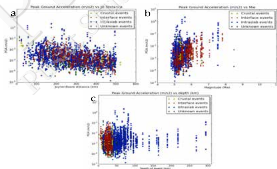
Figure 33. Distribution of PGA (in m/s 2 ) from the records in this study with respect
