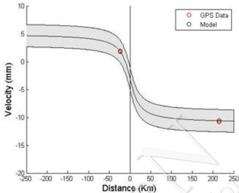
Gambar IV-25. Segmen Musi-Manna
