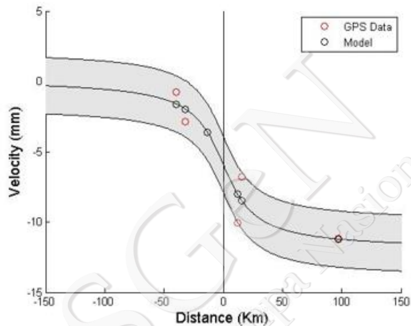
Gambar IV-22. Segmen Sumpur-Sianok-Sumani
