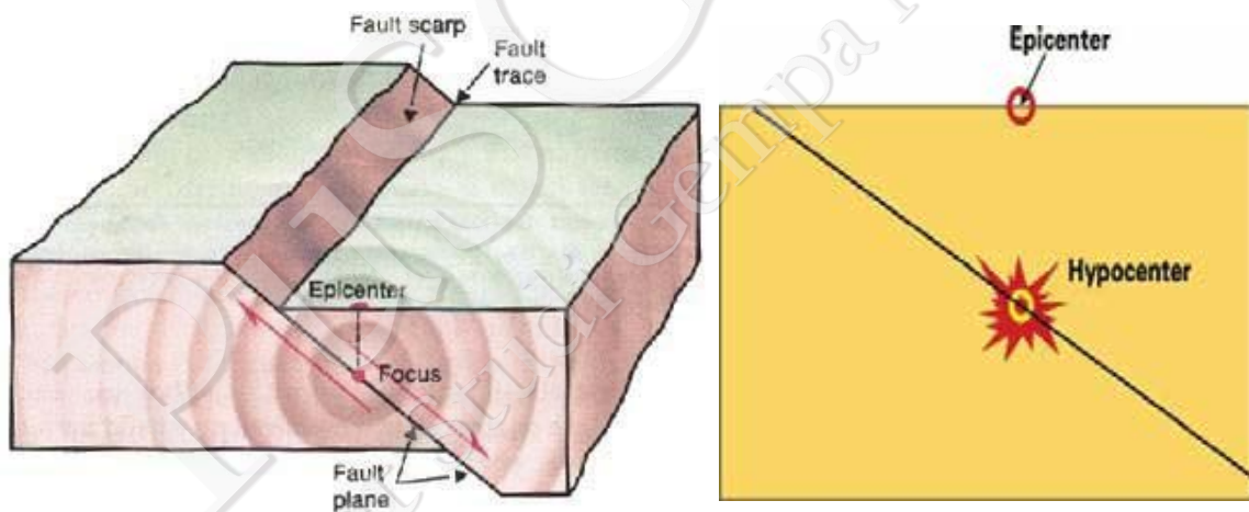
Gambar VI-5. Ilustrasi model sumber gempa sesar/ fault ( http://earthquake.usgs.gov/learn/glossary/ )
